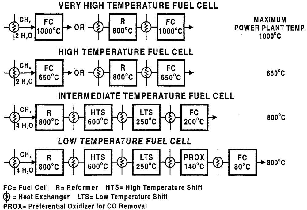
Figure 5. Generic system designs for different types of fuel cells.
