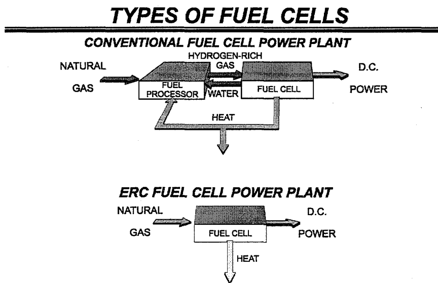
Figure 4. Basic approaches for fuel cell power plants.
