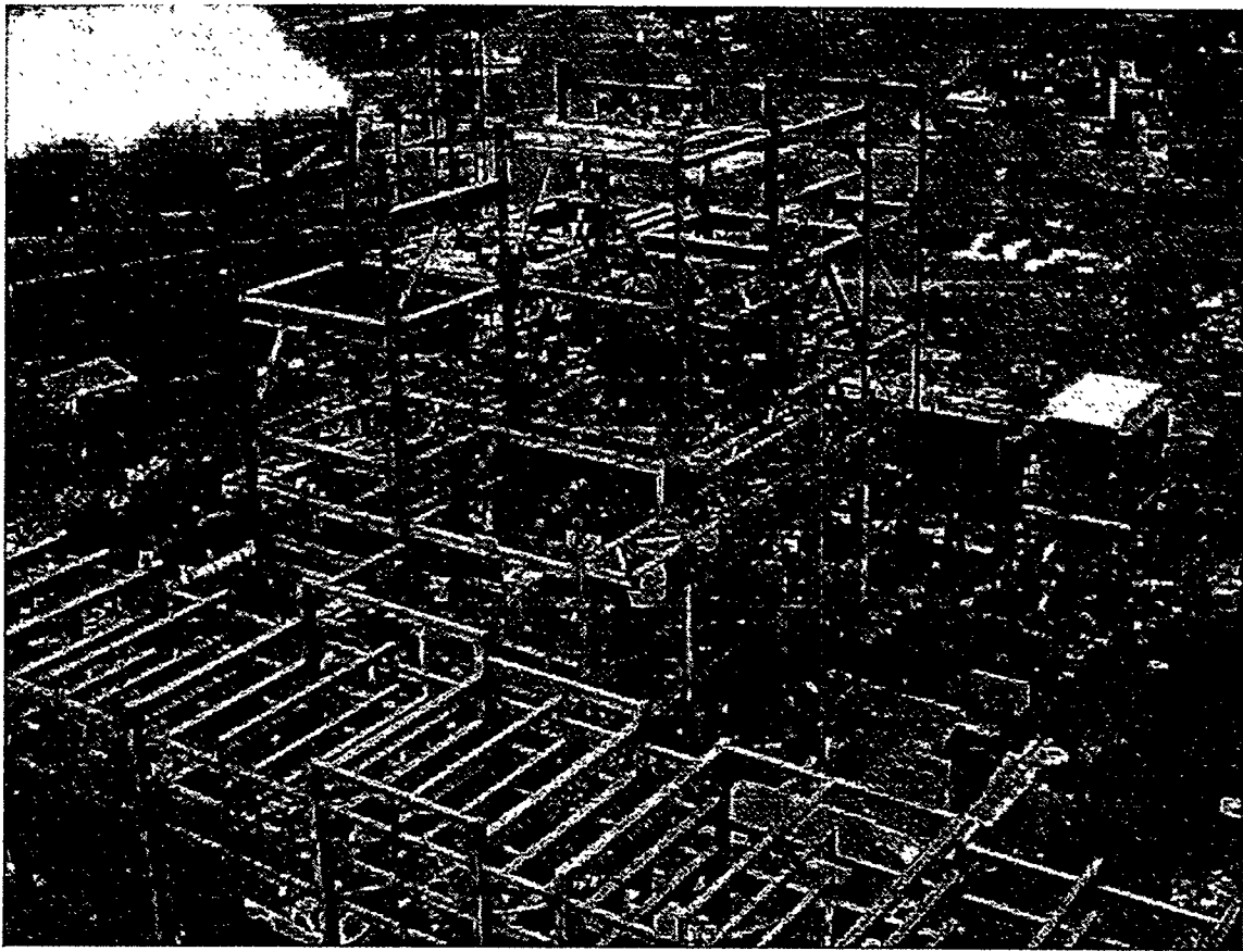
Gasifier Structure to 153' Elevation. Foreground: Piperack. Top Right: Stacker/Reclaimer Foundation.
