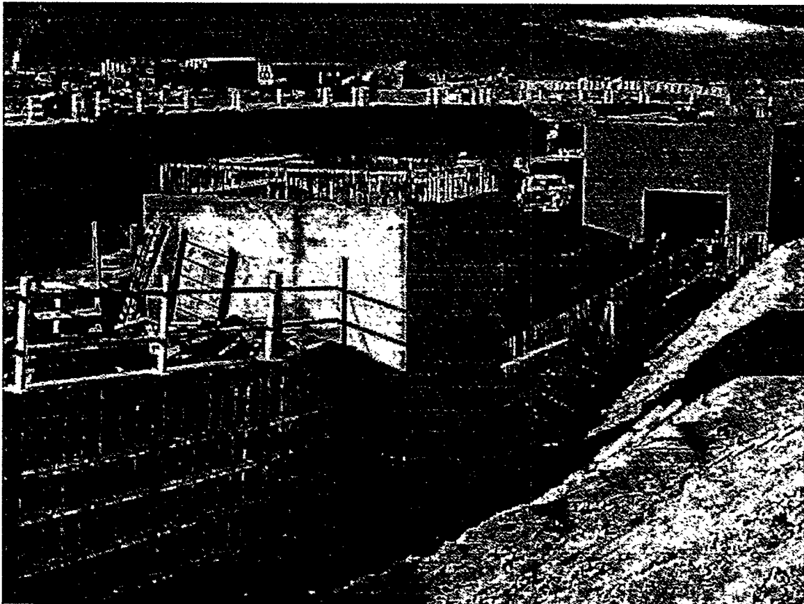
Stacker/Reclaimer Foundation.
