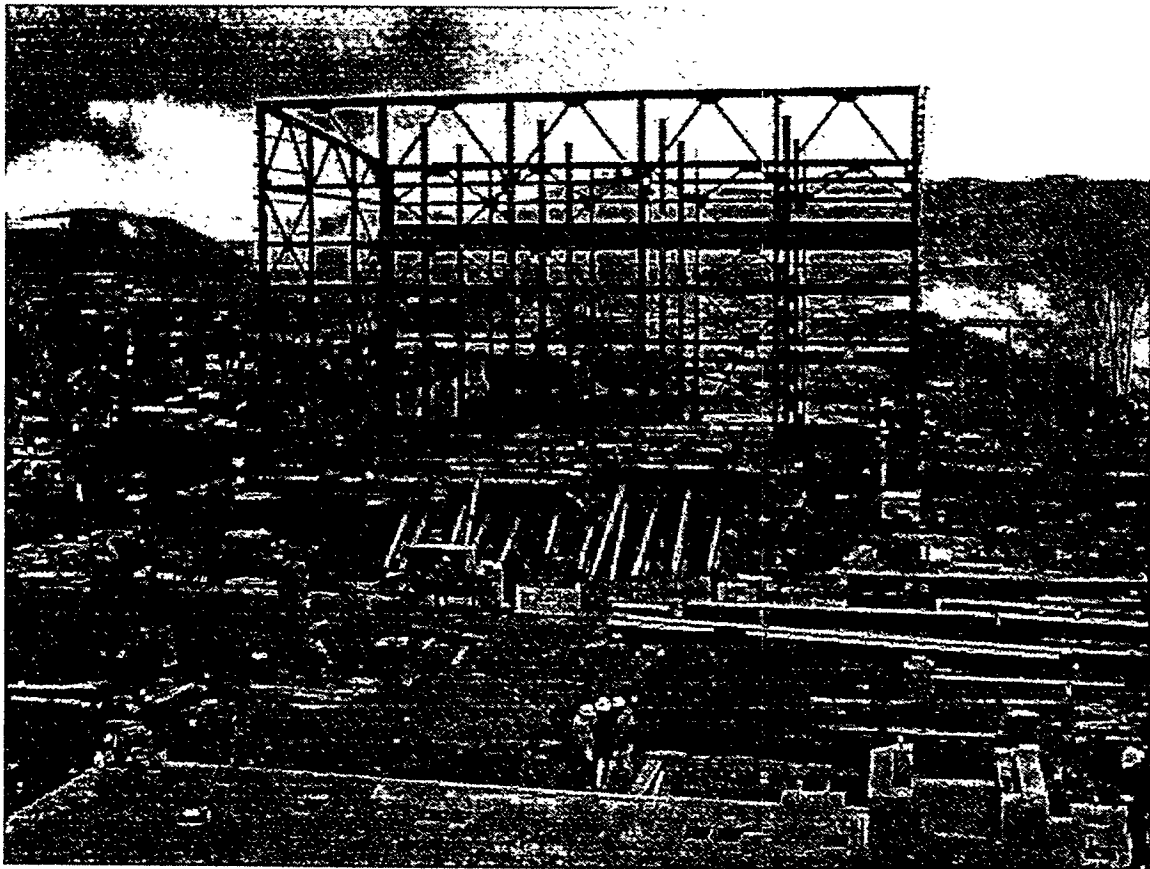
Background: Utility Building Structural Steel. Middle: Steam Turbine Pedestal. Bottom: Gas Turbine Foundation.
