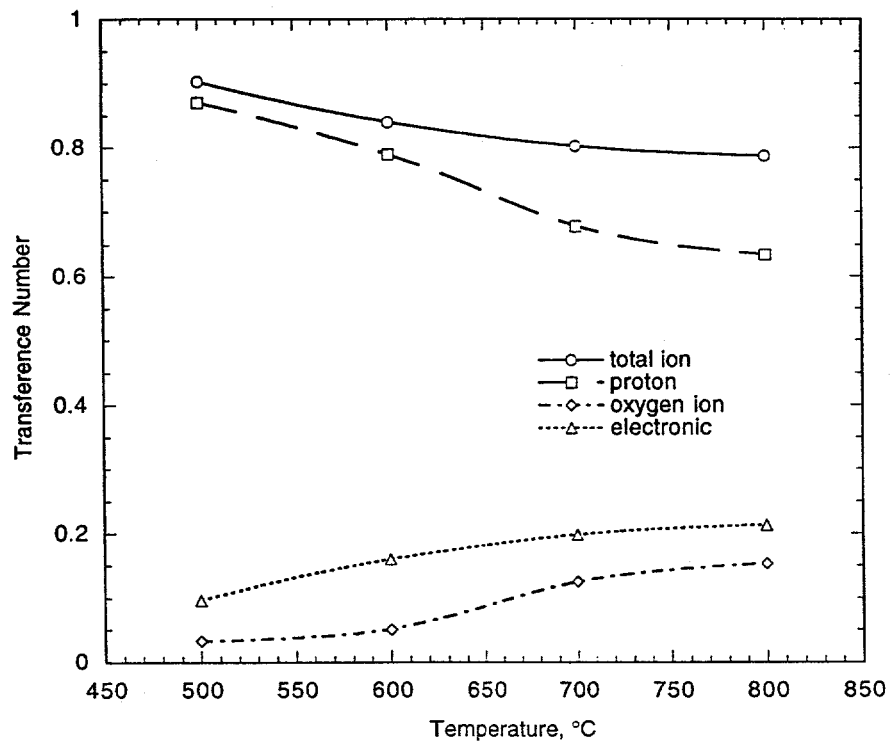
7. Transference numbers of 5% yttria-doped BaCeO 3 samples as determined in hydrogen-containing environments.
