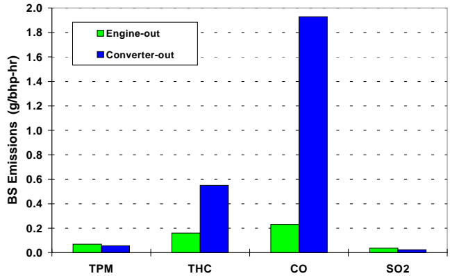
Figure 3.3-4. A comparison of by-product emissions between the converter-out and engine-out with the high-temperature lean-NO x catalyst (Cummins ISM engine, 3-ppm fuel, 4-mode composite)
