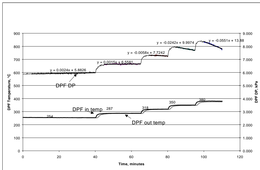
Figure 2.2-2. Example test results from the 5-mode BPT test
