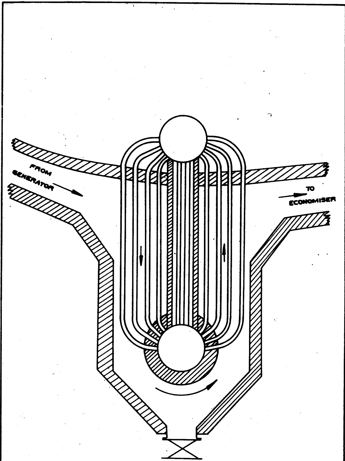
FIG. II. TYPICAL ARRANGEMENT OF WASTE HEAT BOILER
