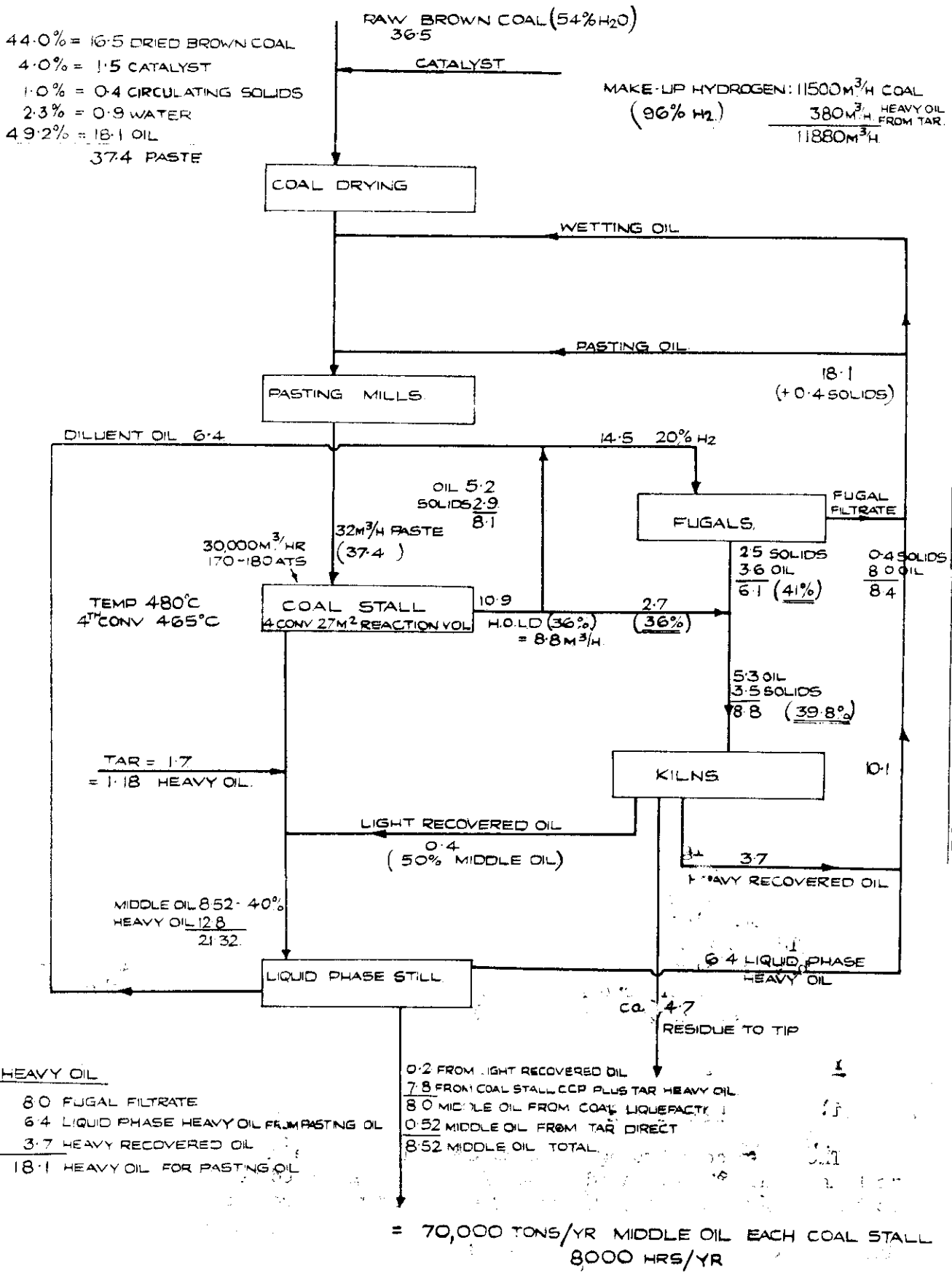
FIG. 11 HYDROGENATION OF BROWN COAL 1944 ALL QUANTITIES IN TONNES/HR EXCEPT WHERE STATED
