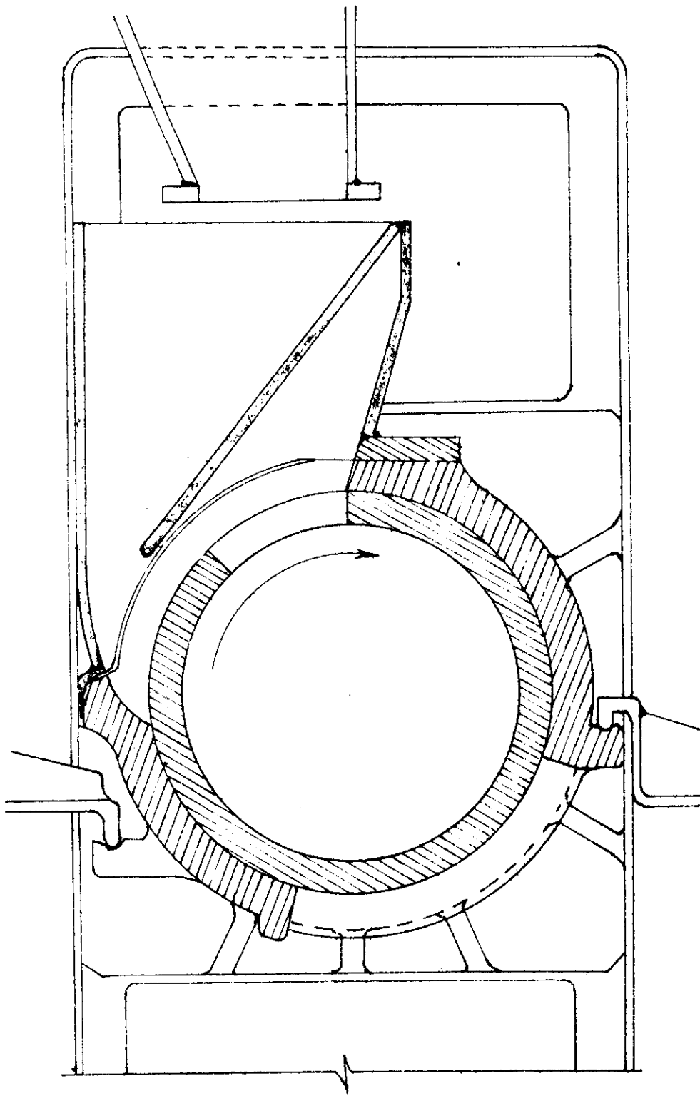
CATALYST VALVE - CATALYTIC CRACKING UNIT
