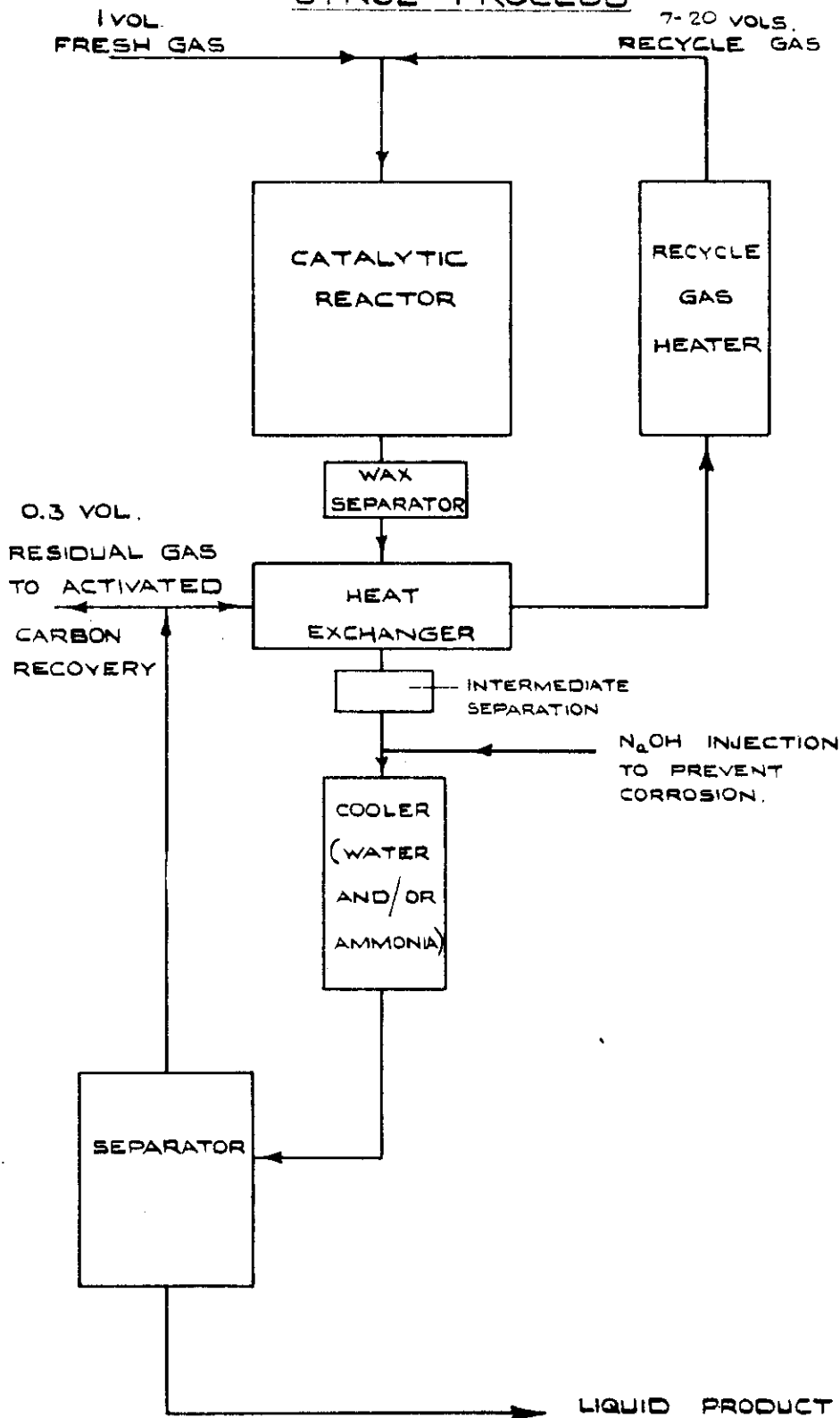
FIGURE XXXII SYNOL PROCESS
