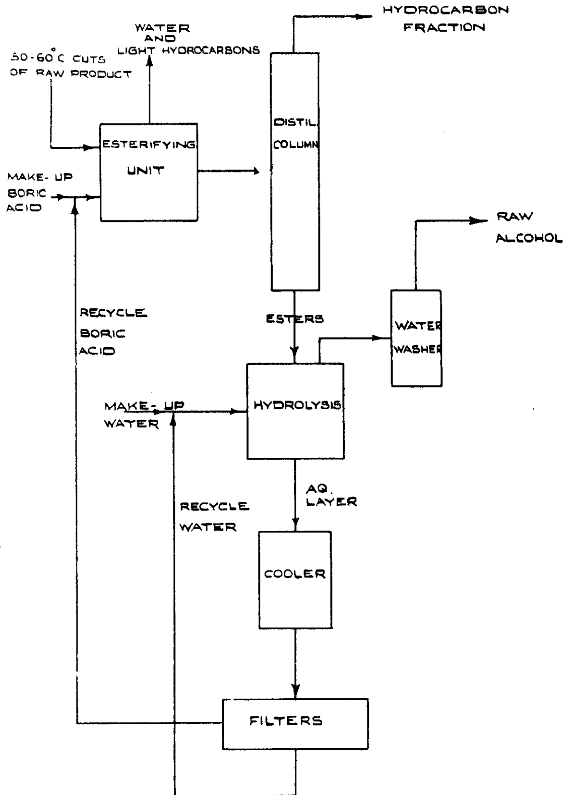
FIGURE XXXVI SYNOL PROCESS - BORIC ACID PLANT
