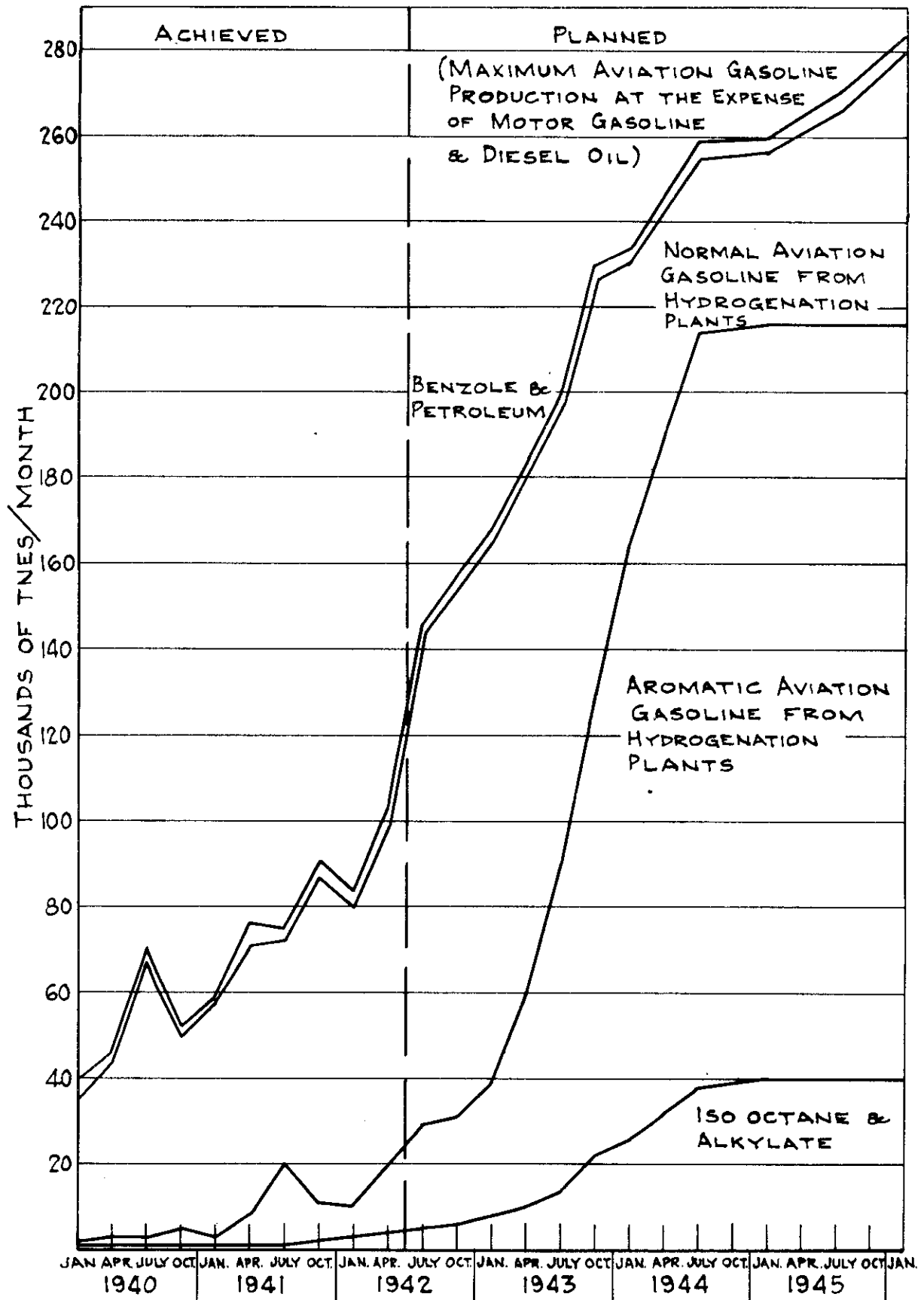
FIGURE XLII.- AVIATION GASOLINE PRODUCTION (MAXIMUM PROGRAMME).
