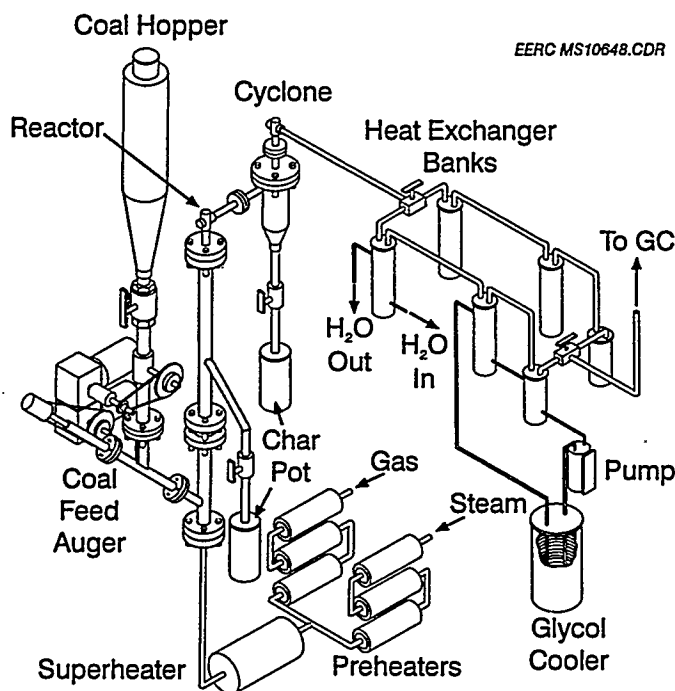
Figure 1. 4-lb/hr CFBR.
