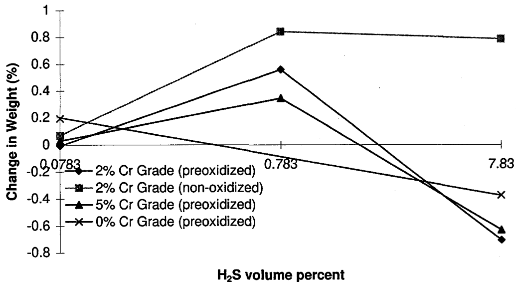
% Change in Weight vs. H 2 S volume percent at 925°F after 14 day exposure and cleaning in IPA
