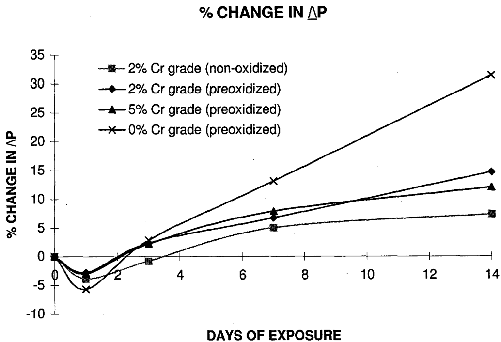
Figure 14. Exposure #3, 925°F with 7.83 vol% H 2 S
