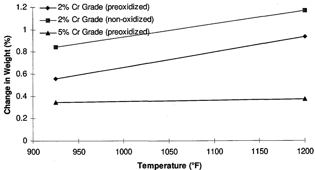
% Change in Weight vs. Temperature at 0.783 vol% H 2 S after 14 day exposure and cleaning in IPA
