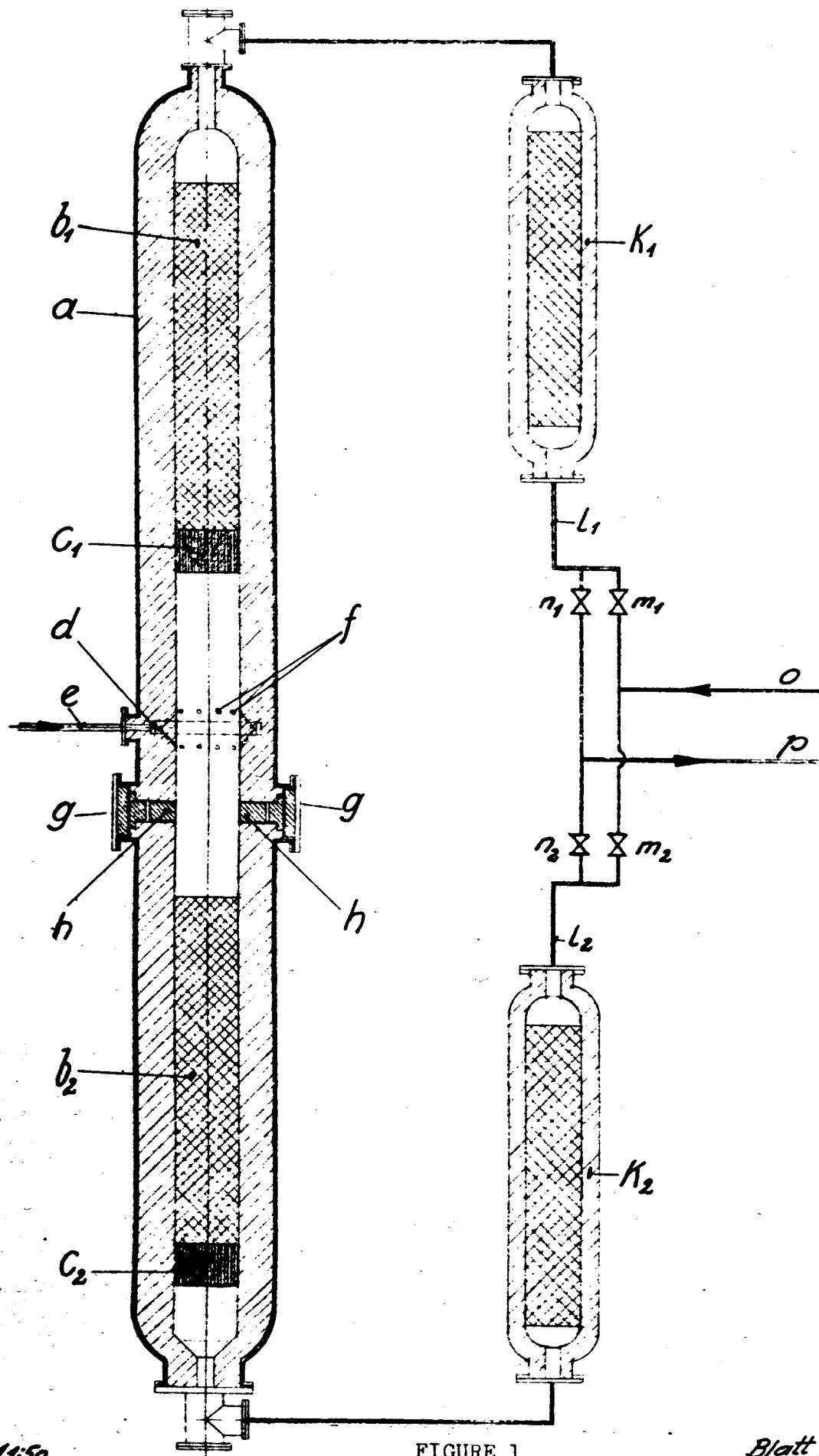
FIGURE 1 SCHMALFELDT METHANE CRACKING PILOT PLANT
