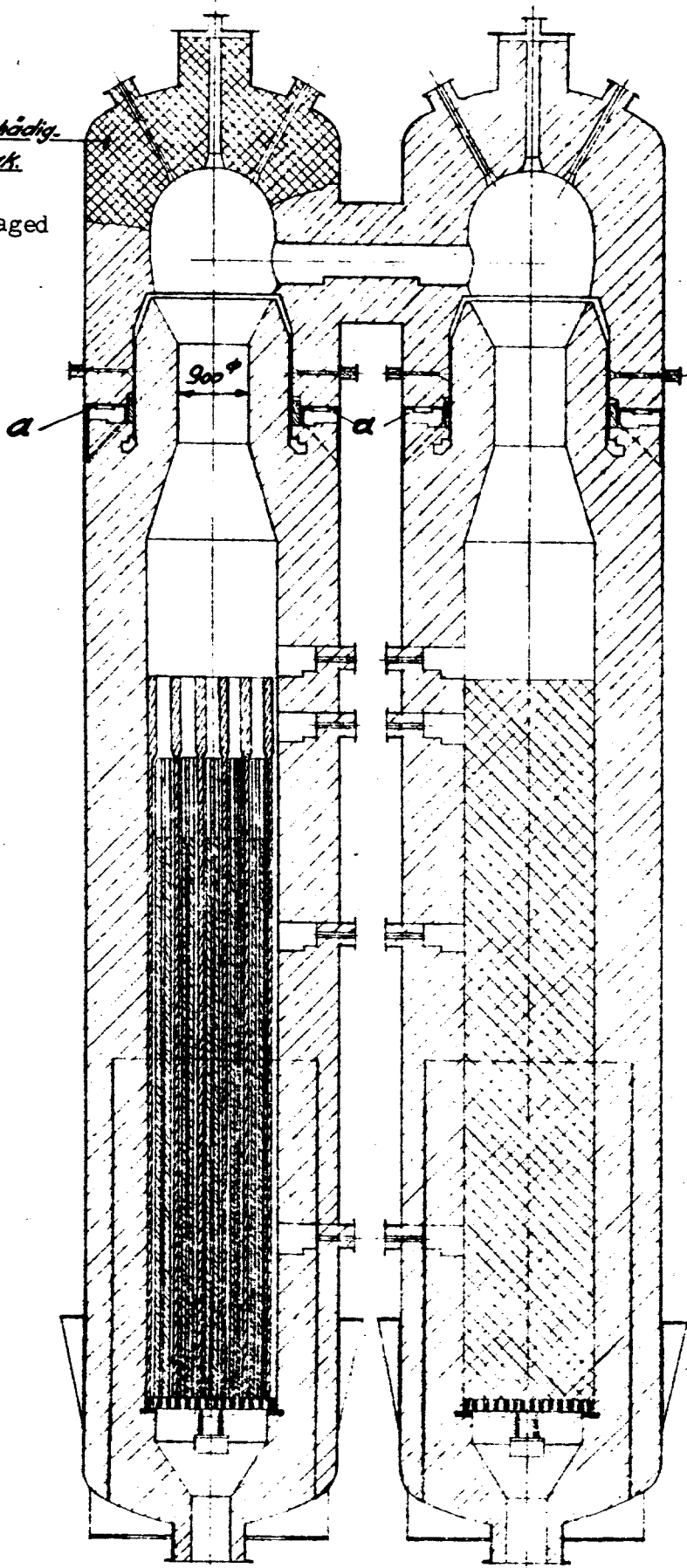
FIGURE 2 LARGE SCALE METHANE CRACKING REACTORS
