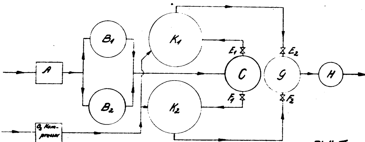
FIGURE 3 LARGE SCALE METHANE CRACKING PLANT LAYOUT
