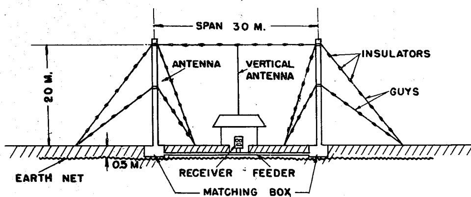
Figure 5 ELEVATION
