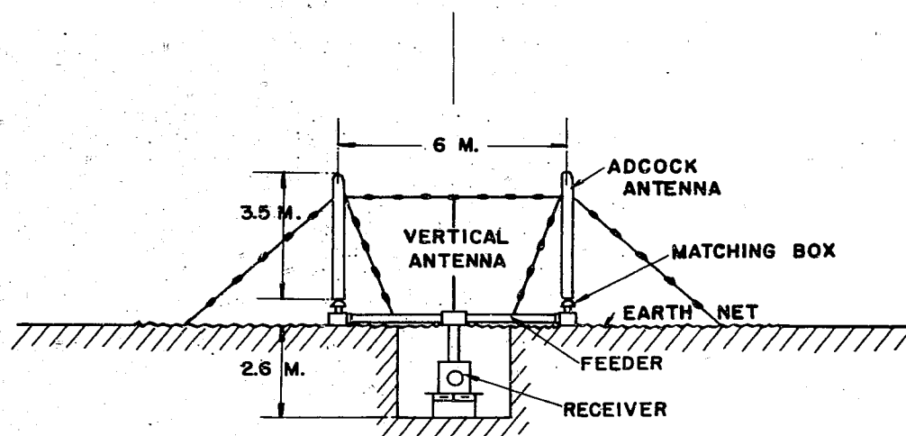
Figure 7 ELEVATION
