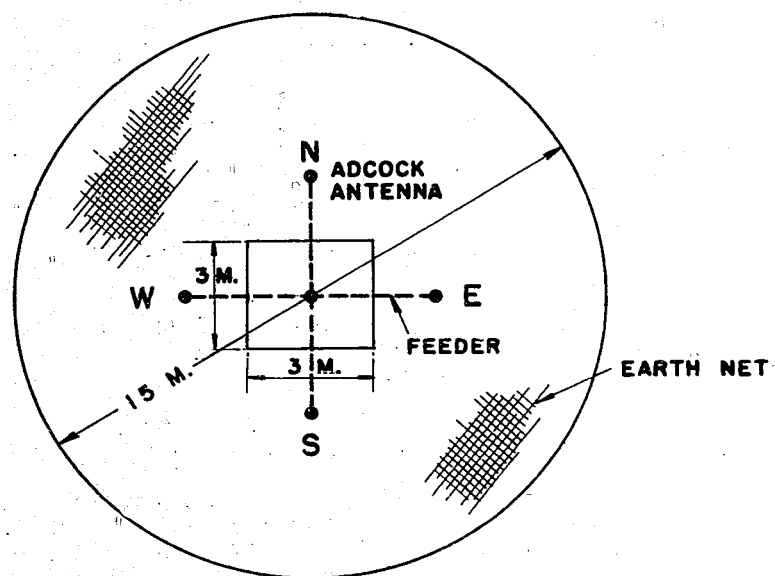
Figure 6 PLAN VIEW
