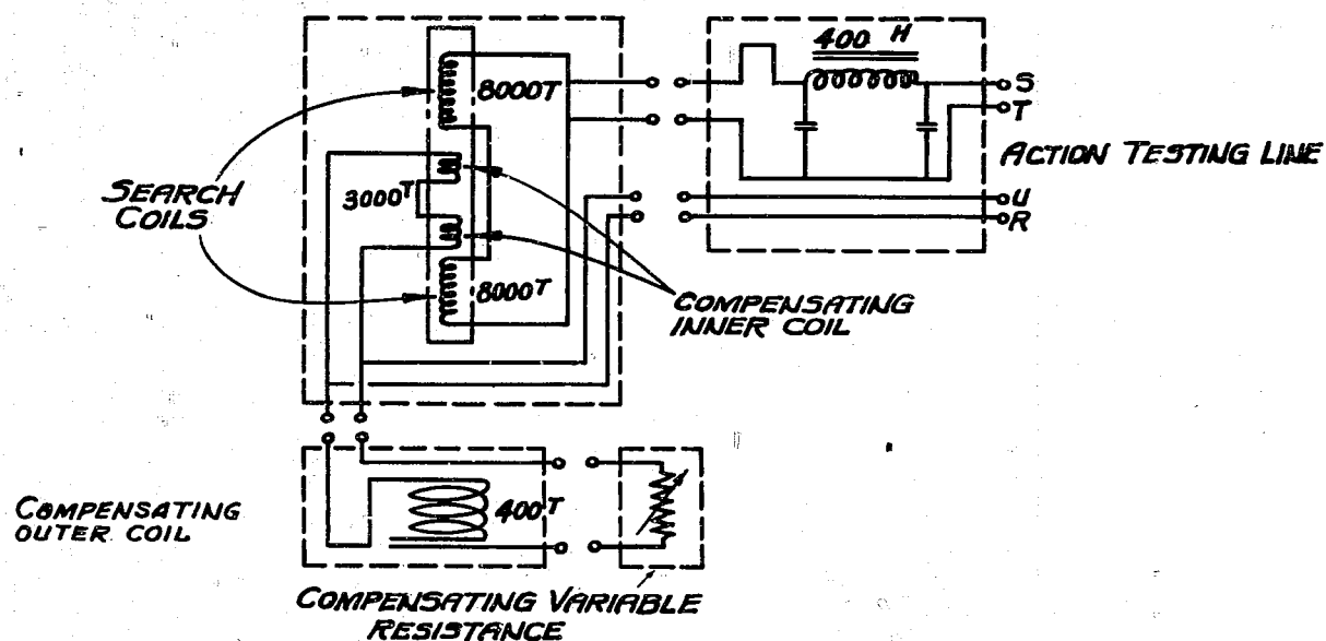
Figure 5 SEARCH COIL, FILTER AND COMPENSATOR
